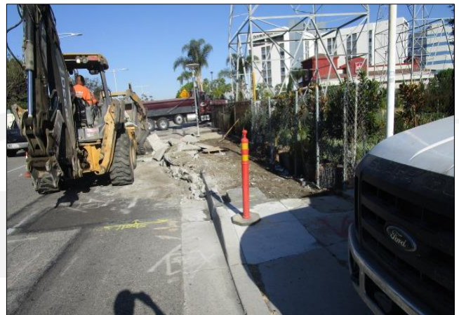
Removing sidewalk on north side west of I-405.
