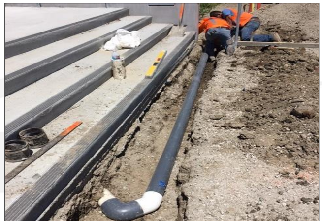
Drainage pipe installation.
