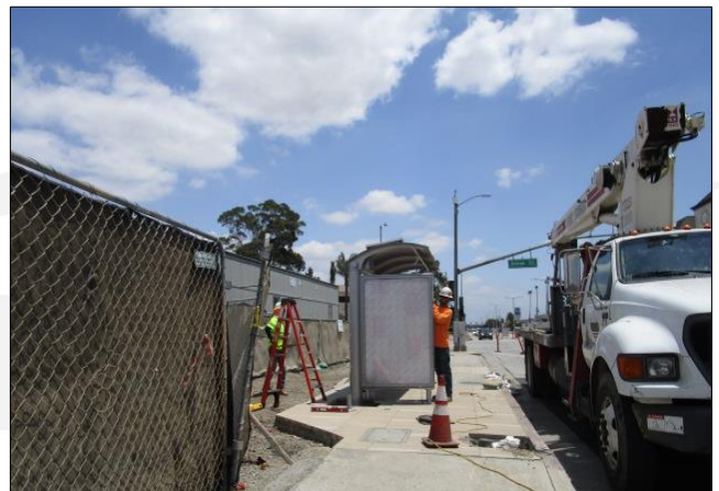
Assembling transit shelter on Carson west of Avalon.
