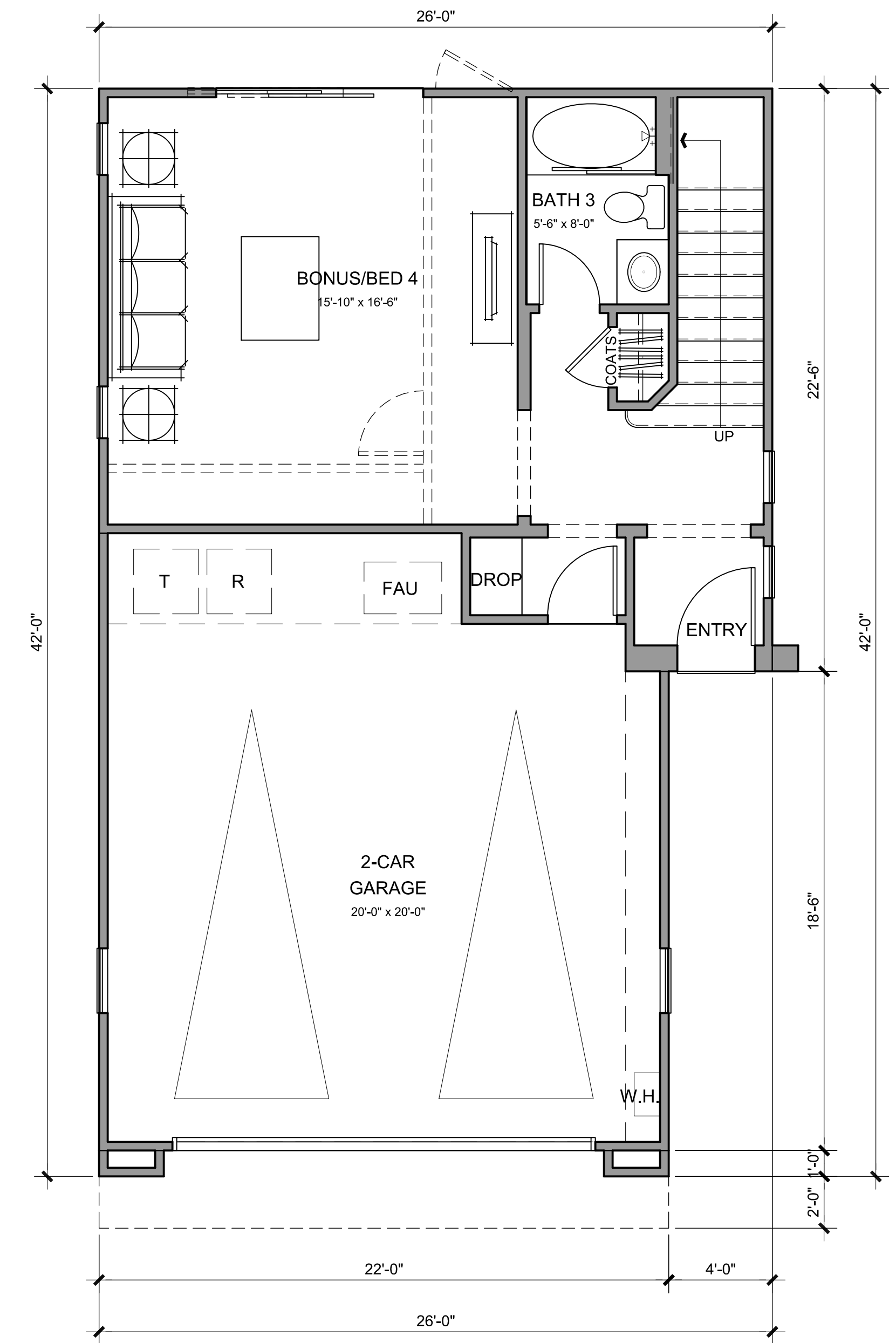
FIRST FLOOR
