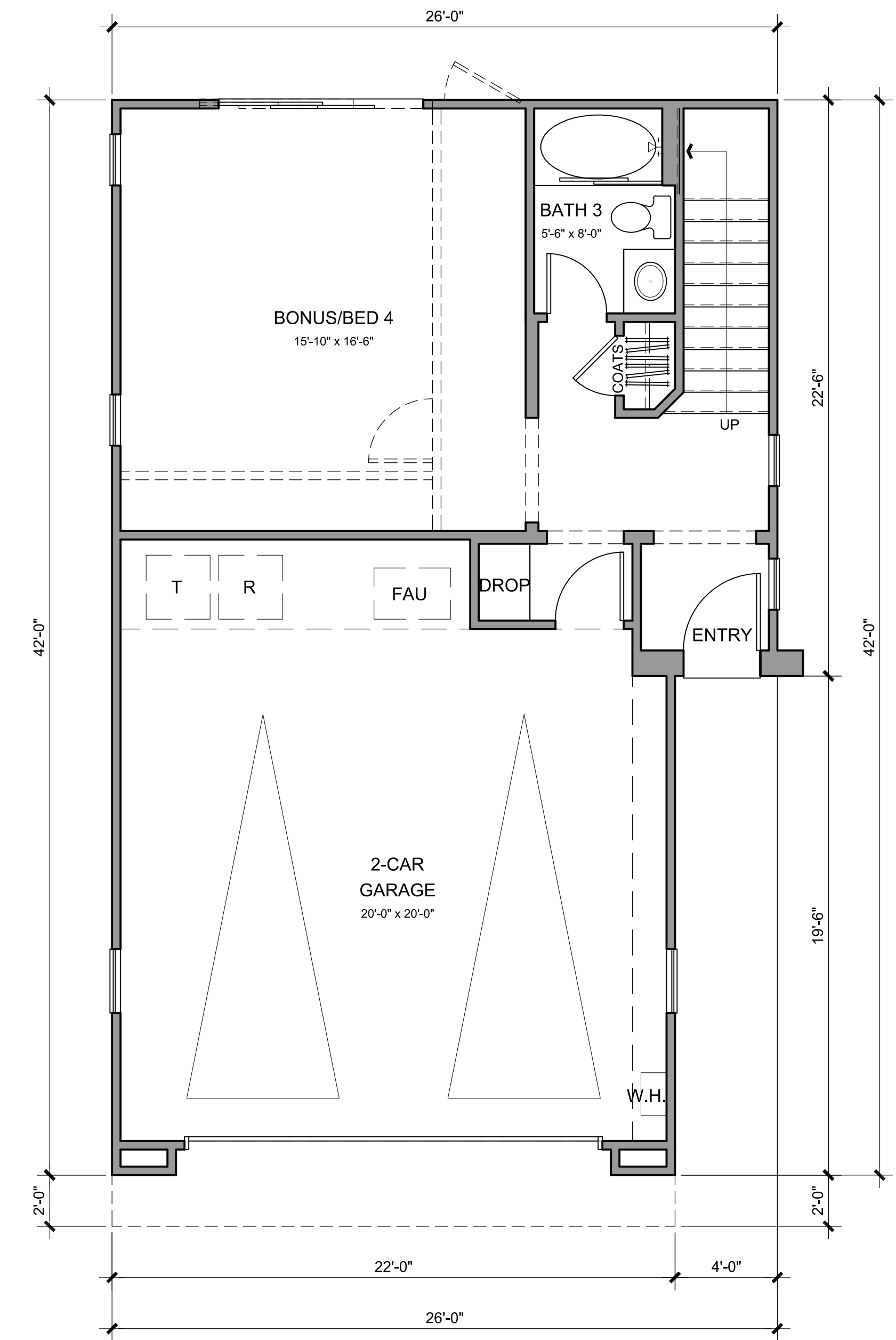
FIRST FLOOR
