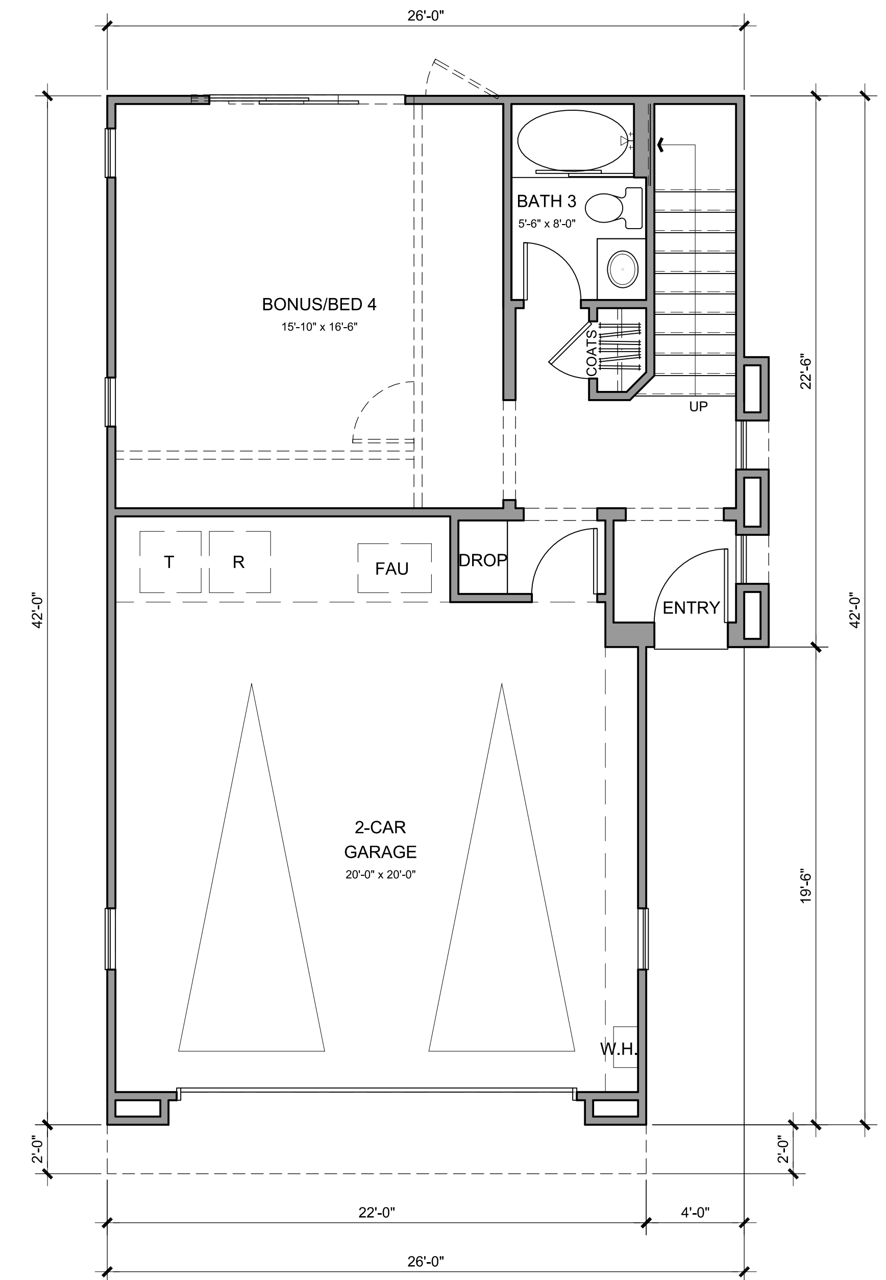
FIRST FLOOR
