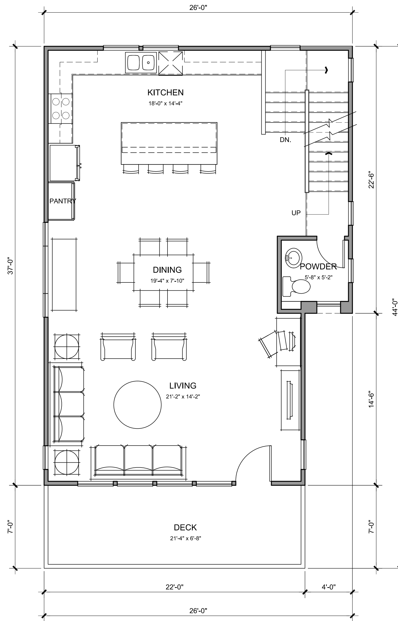
SECOND FLOOR
