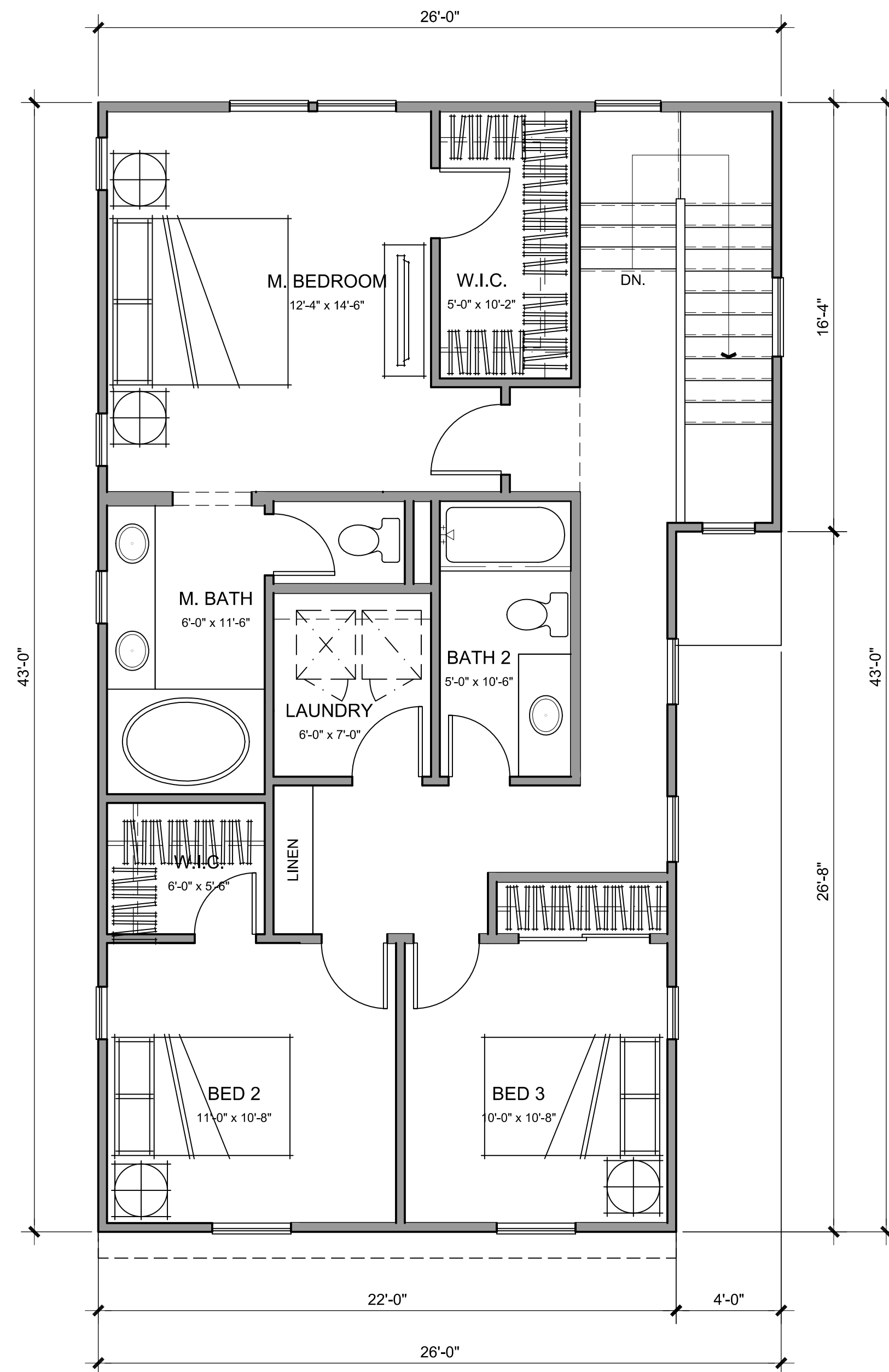
THIRD FLOOR
