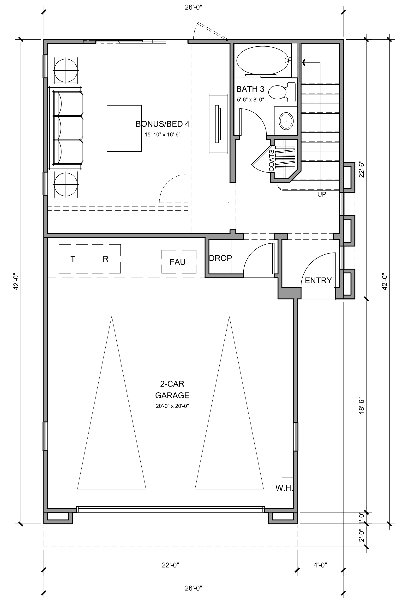
FIRST FLOOR
