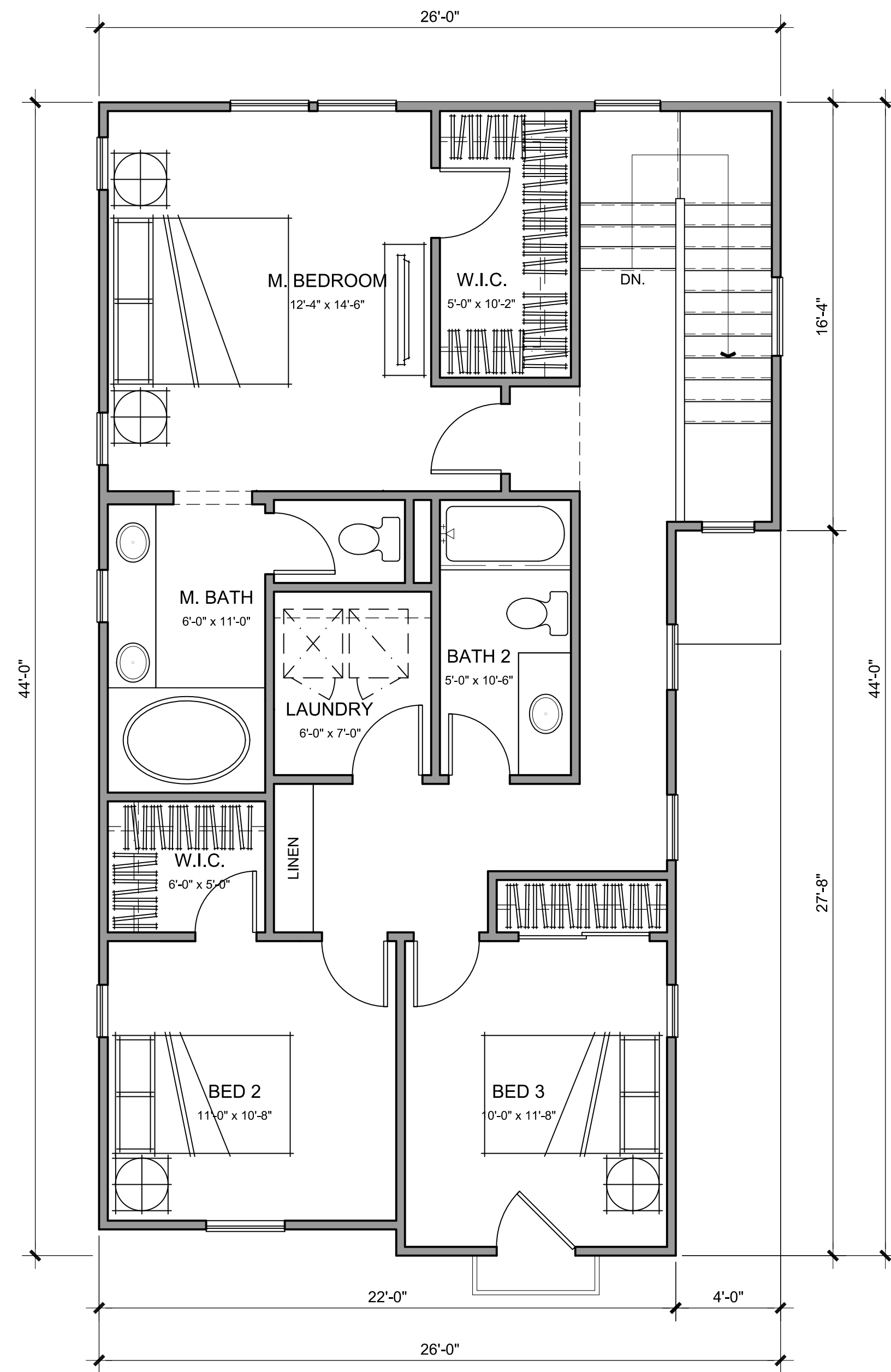
THIRD FLOOR
