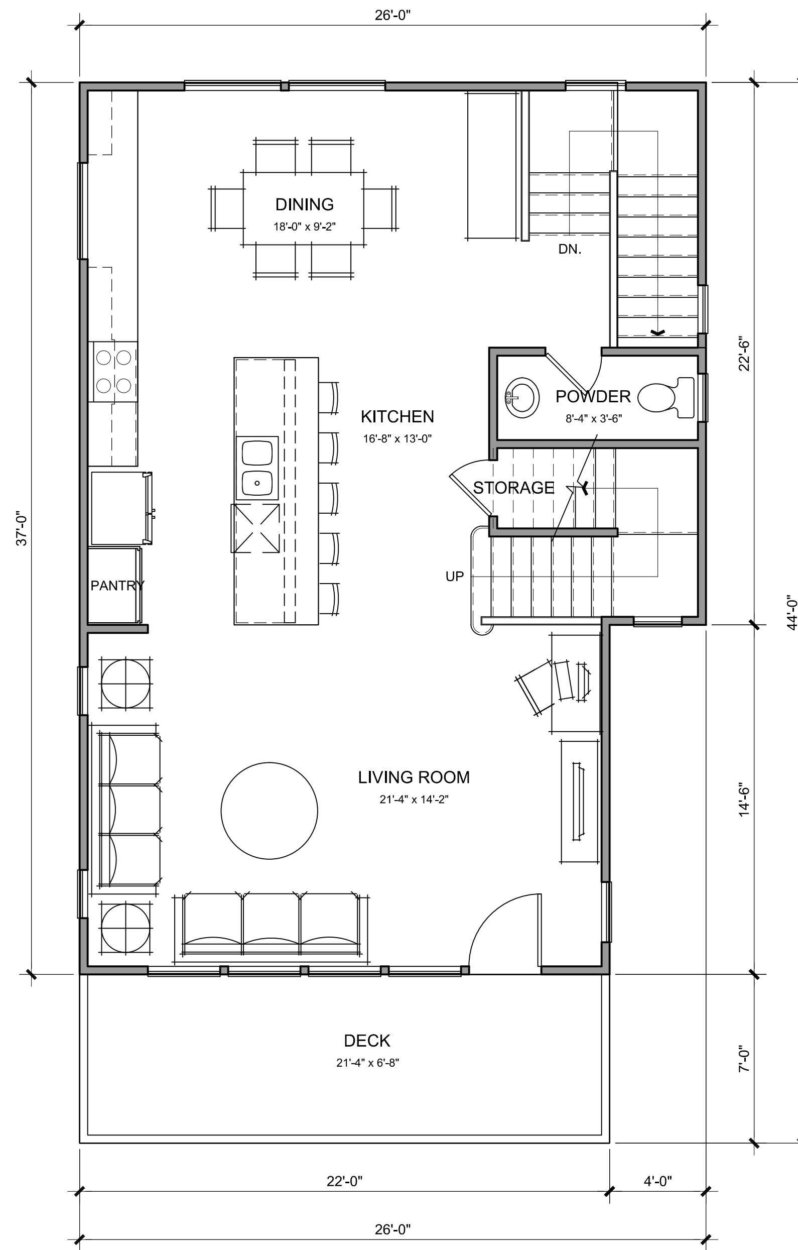
SECOND FLOOR
