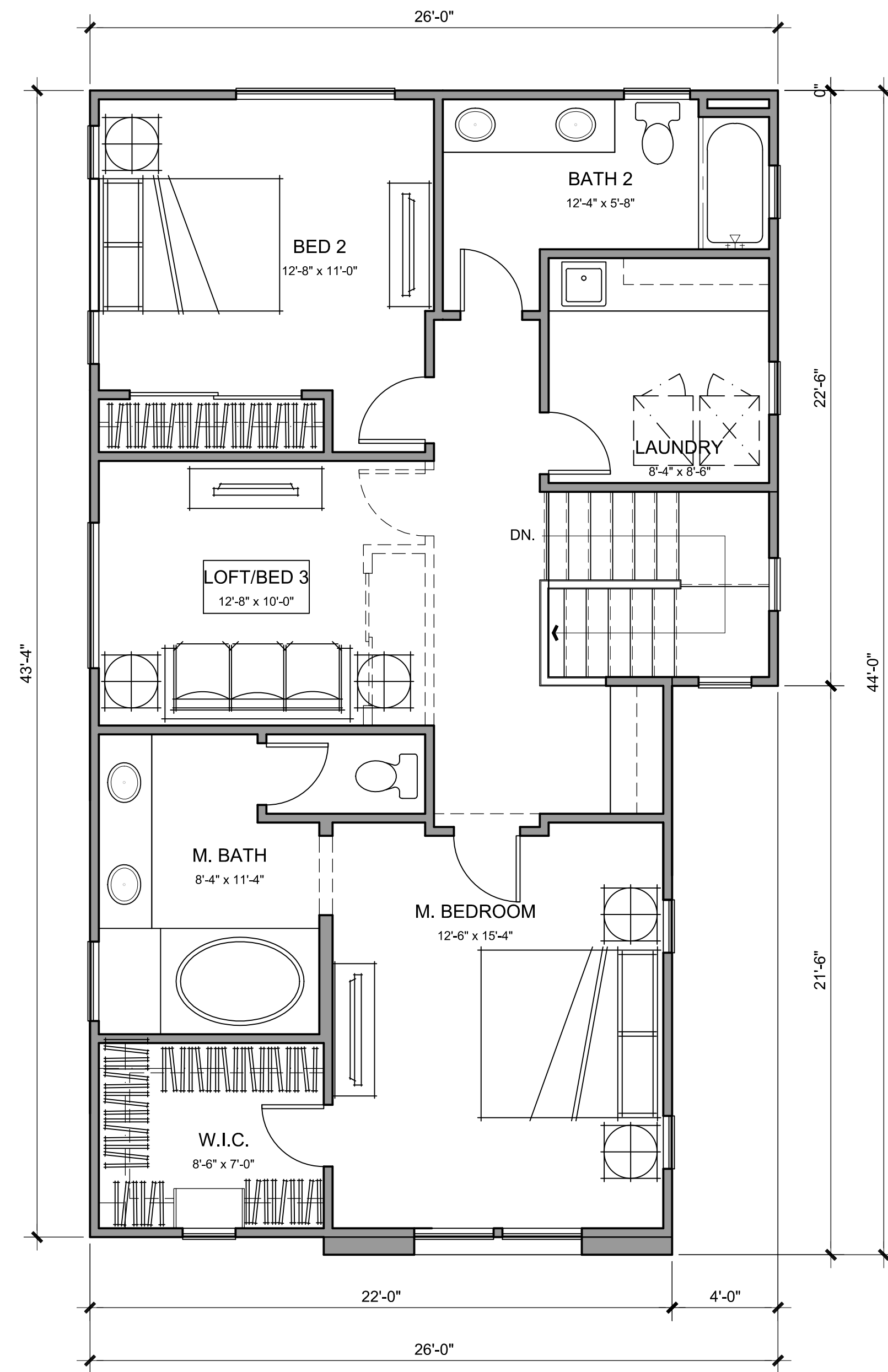
THIRD FLOOR
