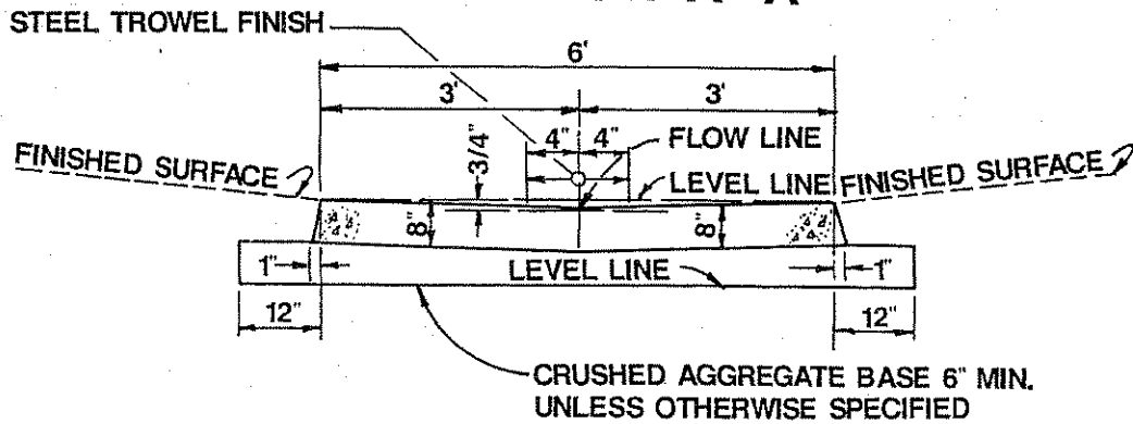
SECTION B-B
