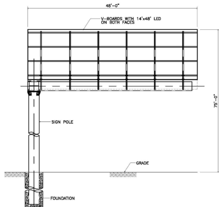
EAST ELEVATION OF PROPOSED V-SIGN 1/8" = 1'-0"
