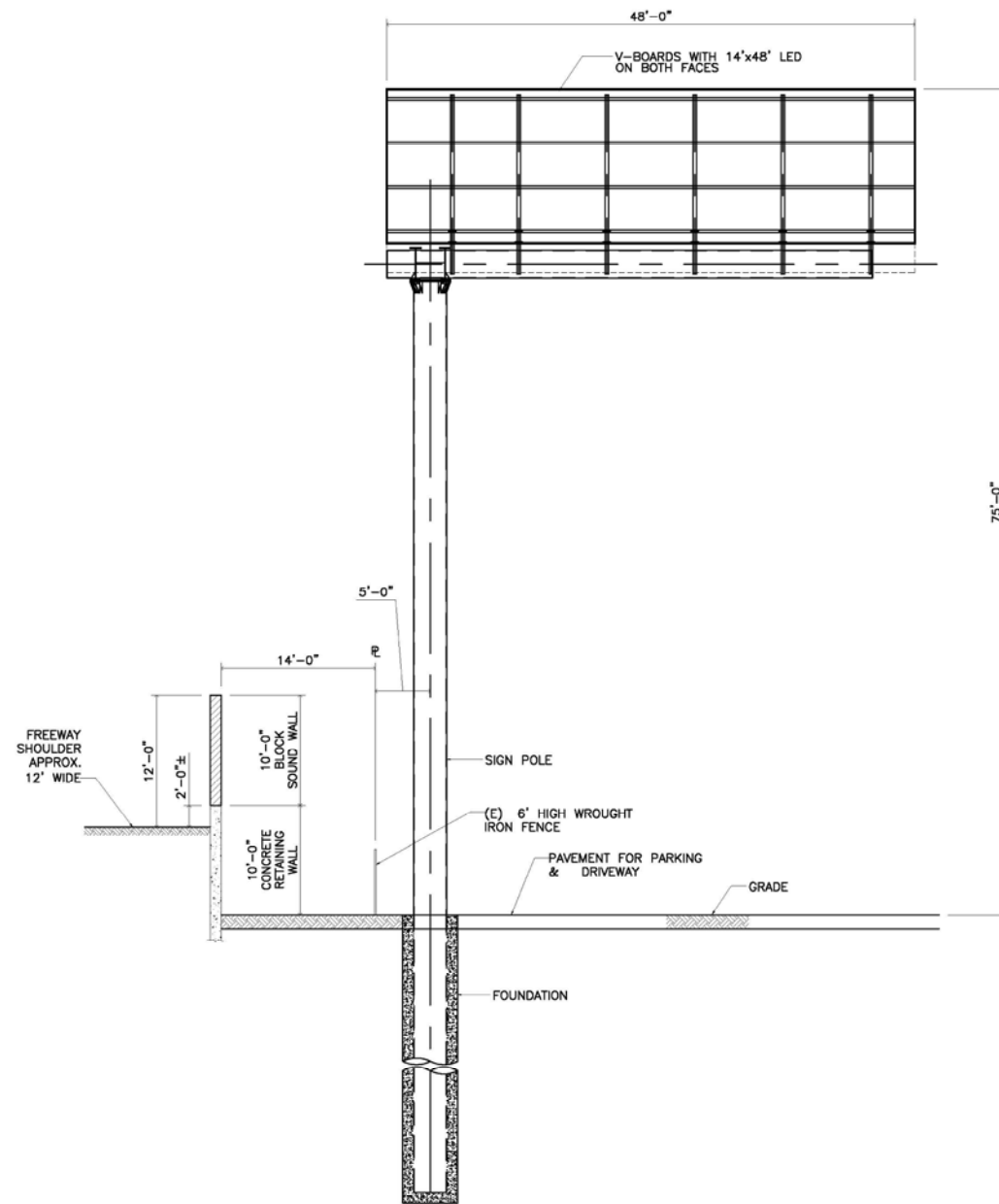
A ELEVATION V-SIGN AND SOUND WALL 1/8" = 1'-0"
