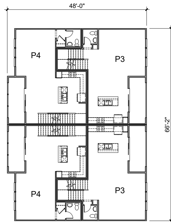
Second Floor 3094 SQ. FT.
