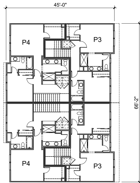
Third Floor 2867 SQ. FT.
