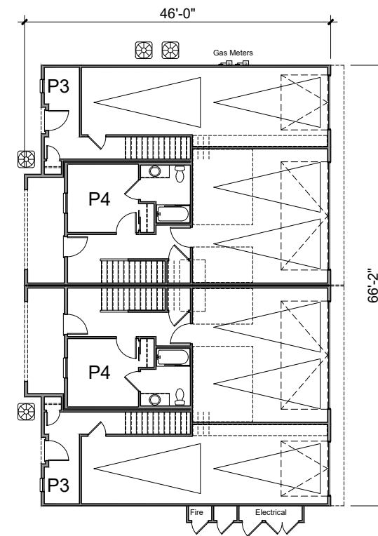
First Floor 3006 SQ. FT.
