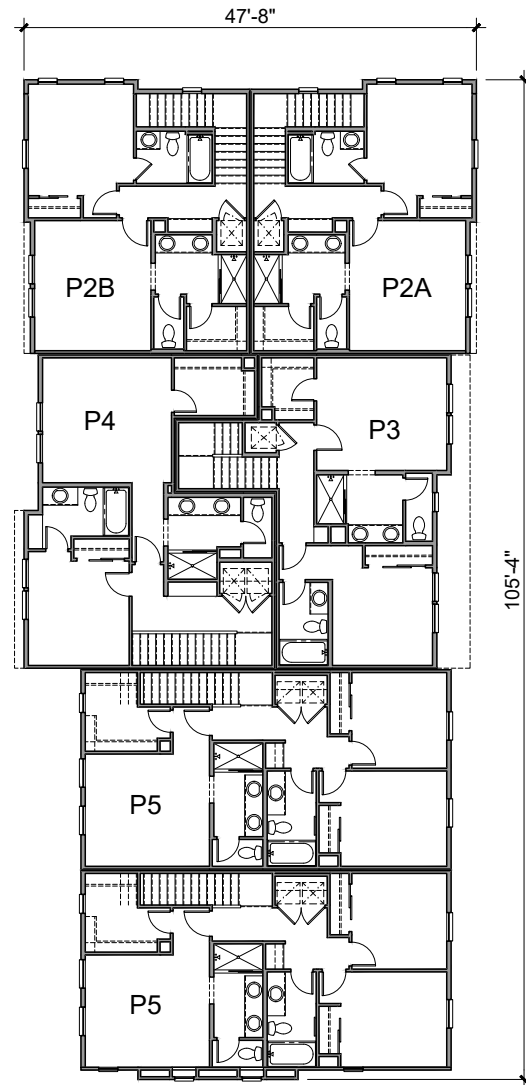
Third Floor 4437 SQ. FT.
