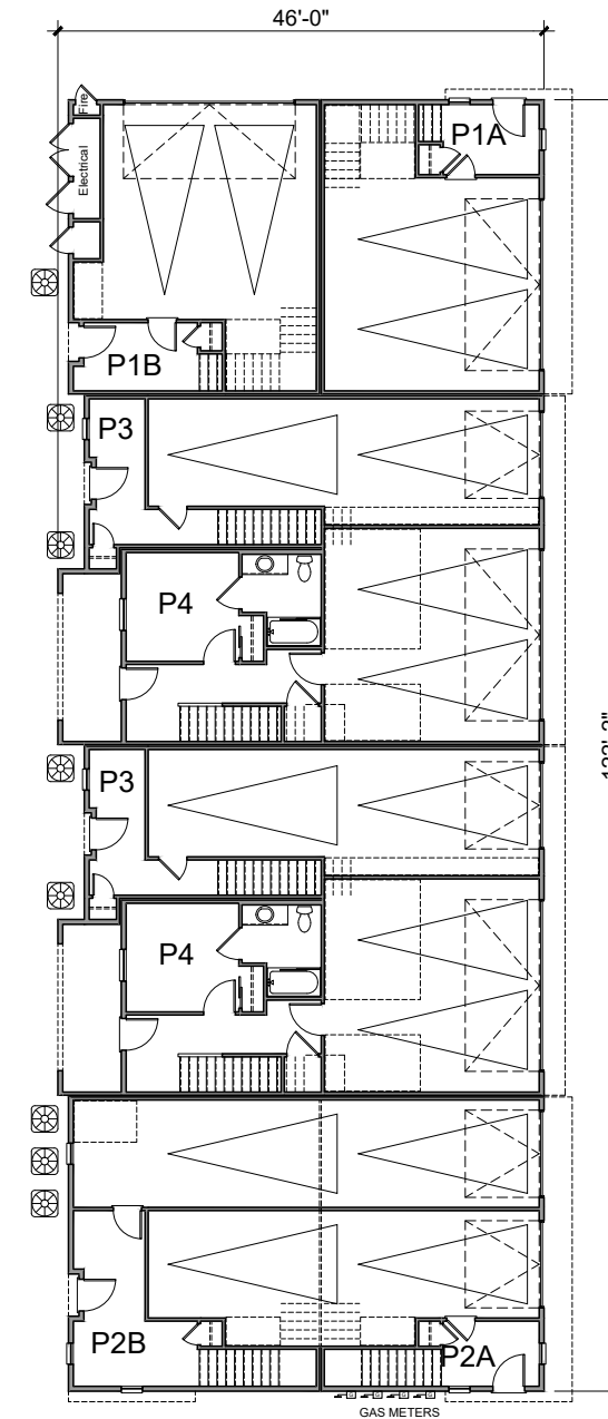
First Floor 5481 SQ. FT.
