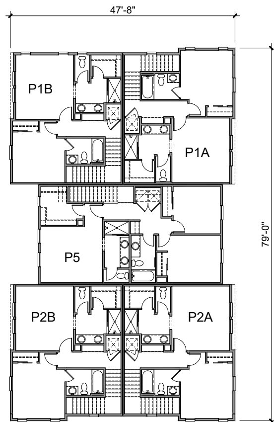
Third Floor 3484 SQ. FT.
