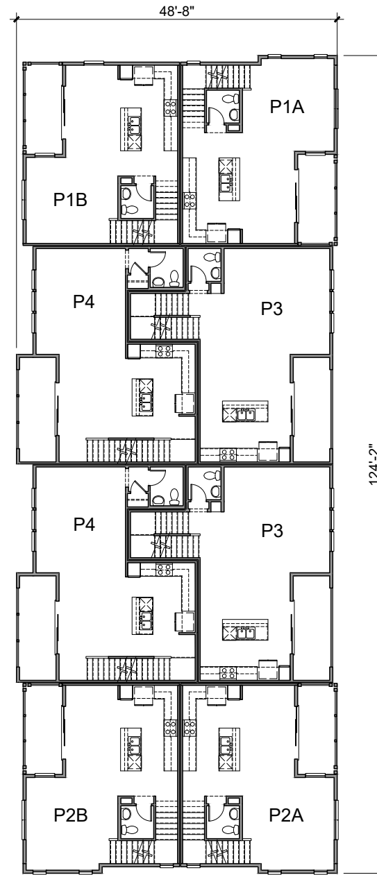
Second Floor 5799 SQ. FT.
