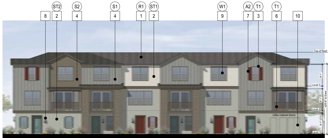
East/West Elevation
